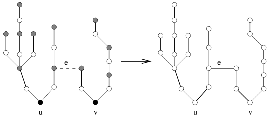
Figure 3.2: Extending a bipartite graph matching
